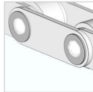
WWS (Welded Washer Selvedge) Rods go through the chain and then retained by a washer welded in place.
