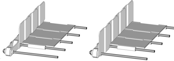
Sideplates on Rod Plate drilled and slide onto rod between slat and chain
